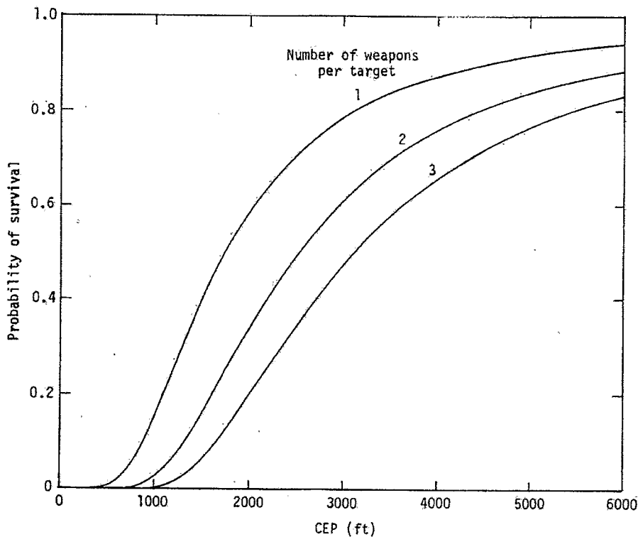
(U) Fig. 7--Probability of survival: effect of multiple shots (2000-psi target; 3-MT weapon yield)
