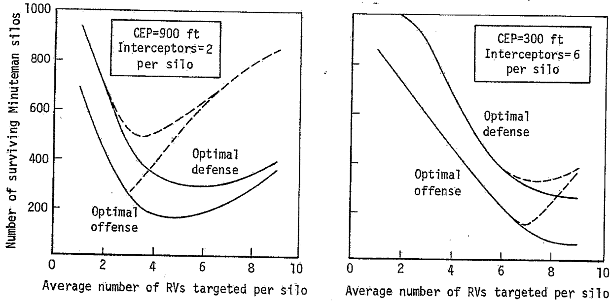
(S) Fig.8—Minuteman hard site defense effectiveness as a function of heavy ICBM MIRV payloads (U)
